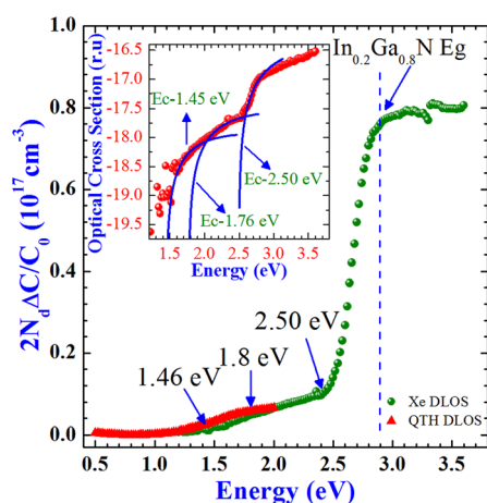
FIG. 3. (Color online) QTH and Xe lamp DLOS measurement on Au/Ag/In 0.2 Ga 0.8 N Schottky diode. Inset shows the optical cross section spectrum in relative units (r.u.) obtained from the slope of the transient analysis.
