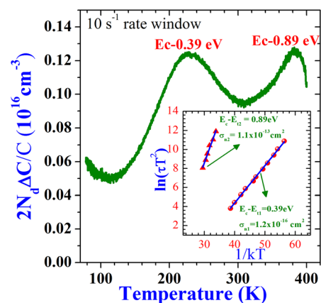
FIG. 2. (Color online) DLTS spectrum of the Au/Ag/ \text{In}_{0.2}\text{Ga}_{0.8}\text{N} Schottky diode for the 10 \text{ s}^{-1} rate window. Inset shows Arrhenius plot for the two defect levels observed in the measurement.
