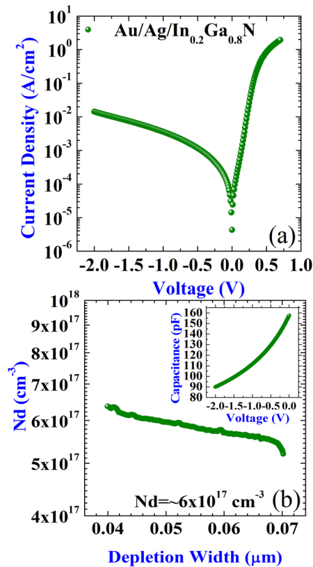
FIG. 1. (Color online) (a) I - V and (b) C - V characteristics of the Au/Ag/ \text{In}_{0.2}\text{Ga}_{0.8}\text{N} Schottky diode.
